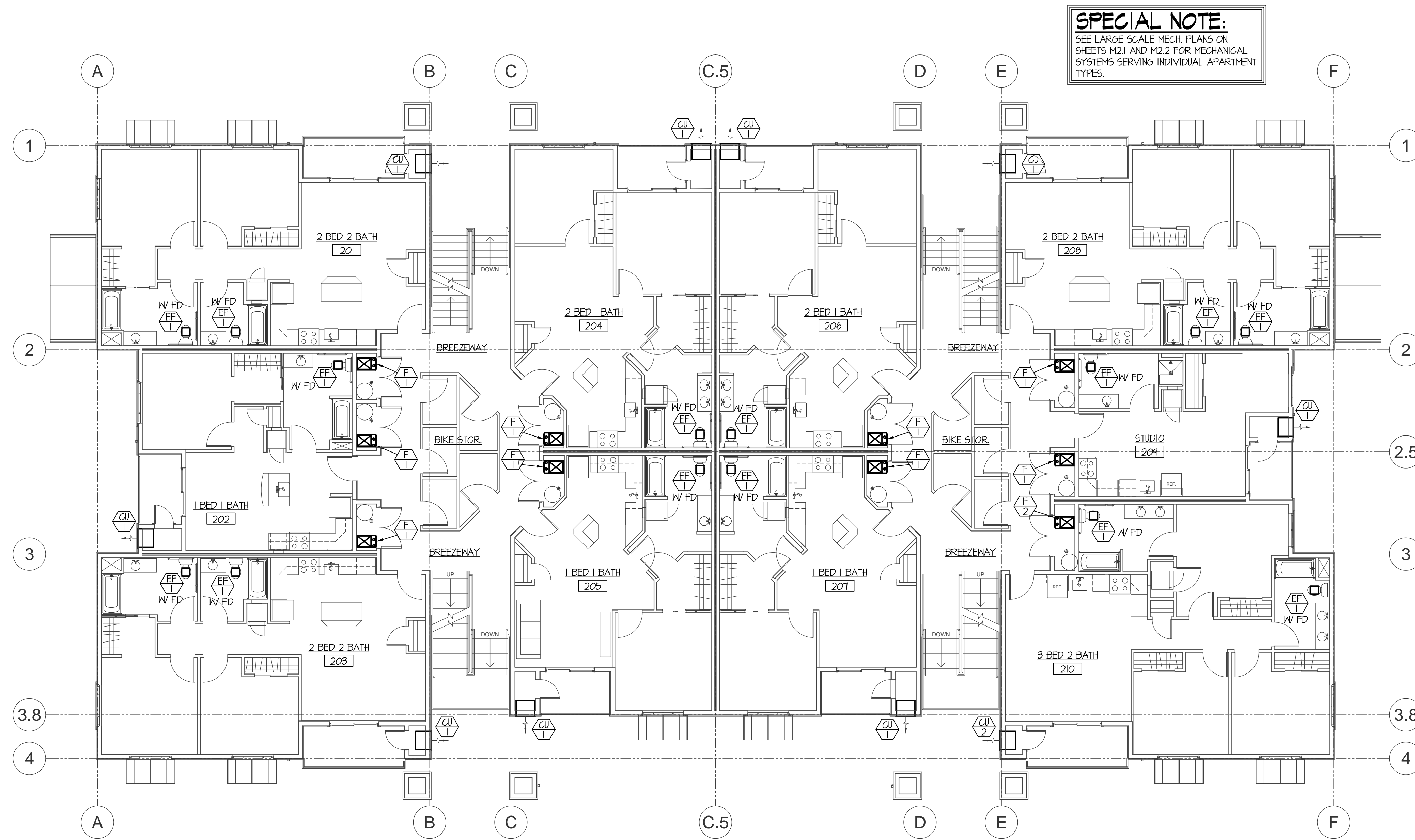
LEVEL 2 MECHANICAL FLOOR PLAN SCALE: 1/8" = 1'-0"
